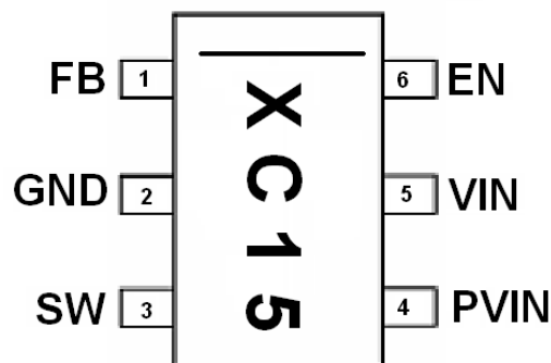
FS1403 / SOT26L
