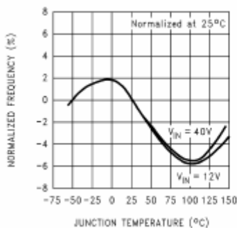
Oscillator Frequency
