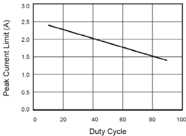
Peak Current Limit vs. Duty Cycle
