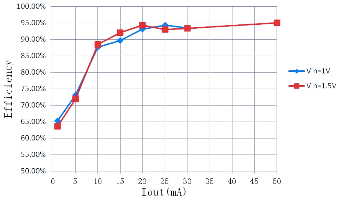
Iout VS Efficiency
