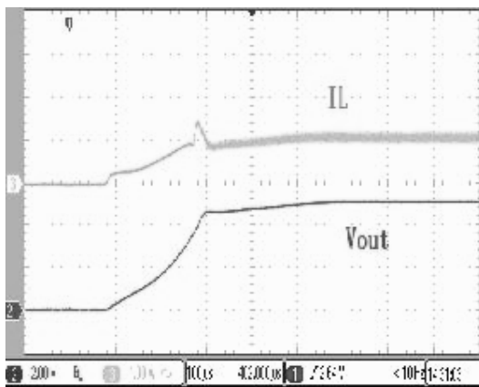
Figure 3. Startup Waveform
