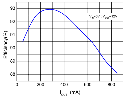
Figure 2: Efficiency Curve
